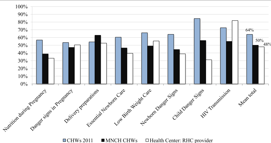
Figure 1 Comparison of MNCH knowledge: (1) self-identified CHWs from 2011, (2) MNCH CHWs, and (3) reproductive child health providers in health centers.
